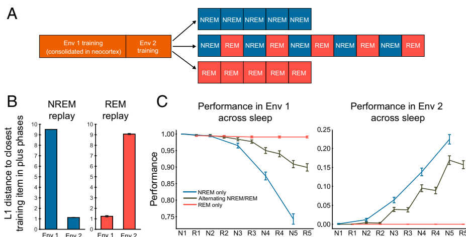
Fig. 4. Simulation 2: Continual learning via alternating sleep stages. (A) Simulation protocol. (B) L1 distance of plus phase attractors to Env 1 and Env 2 item patterns in REM and NREM. Smaller distance indicates more replay of those patterns. (C) Mean performance across sleep for Env 1 and Env 2 items for NREM-only vs. alternating NREM/REM (N/R) vs. REM-only conditions.
